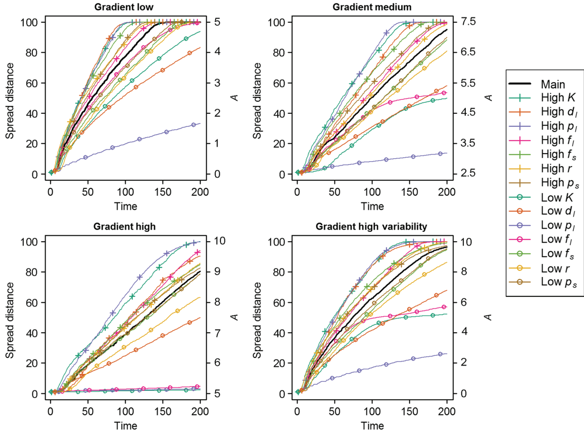
Figure 4. Mean spread trajectories showing sensitivity to model parameters for gradient landscapes. For reference, the right-hand y-axis indicates values of the Allee threshold.
